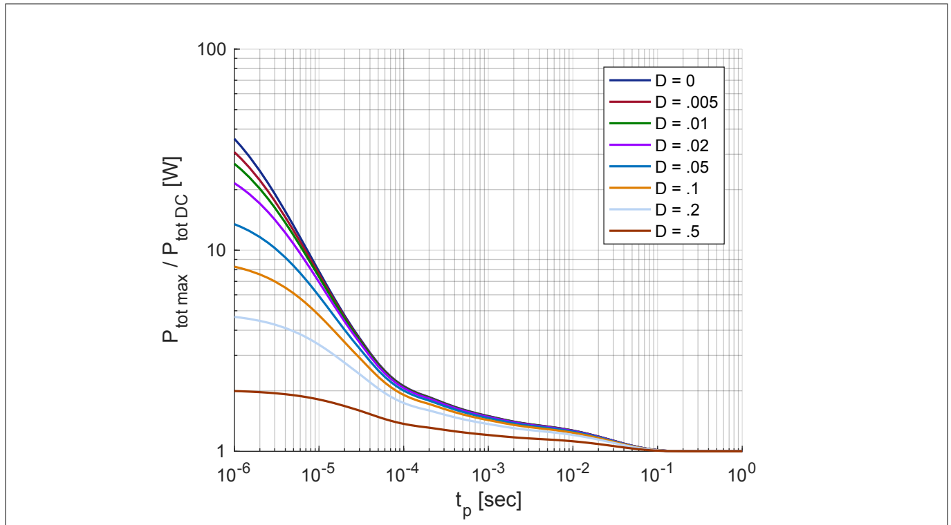
Figure 3 Permissible Pulse Load P_{\text{totmax}} / P_{\text{totDC}} = f(t_p)
