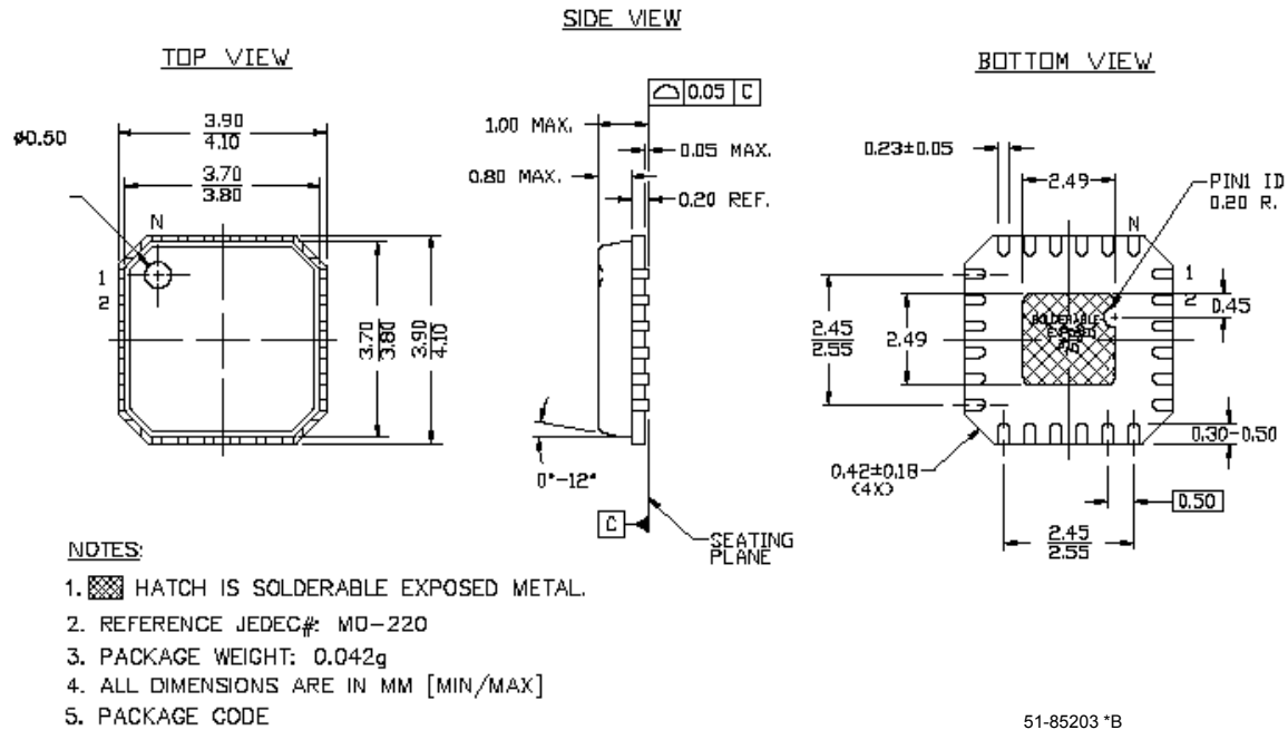
Figure 6. 24-LD QFN 4x4 mm (Subcon Punch Type Pkg with 2.49x2.49 EPAD) LF24A/LY24A
