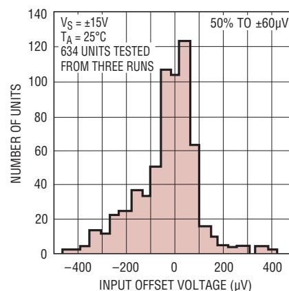
Distribution of Input Offset Voltage (H Package)
