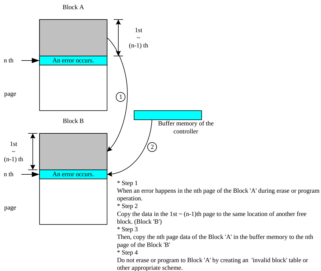
Figure 9.5 Blcok Replacement
