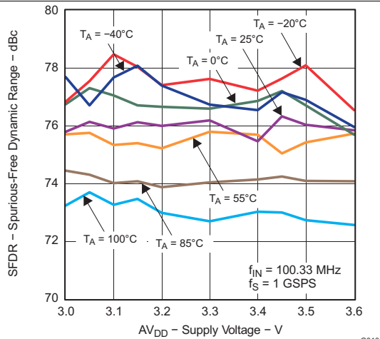
Figure 18. SFDR vs AVDD3 Across Temperature
