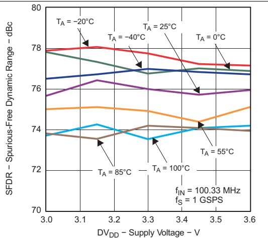
Figure 20. SFDR vs DVDD3 Across Temperature
