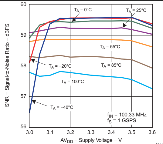
Figure 19. SNR vs AVDD3 Across Temperature
