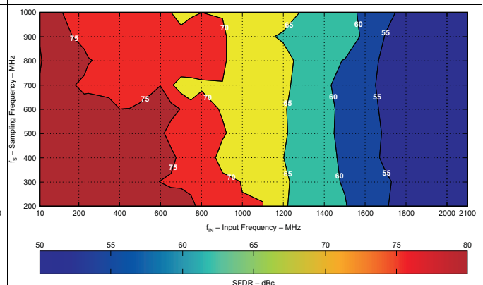
Figure 23. SFDR vs Input Frequency and Sampling Frequency
