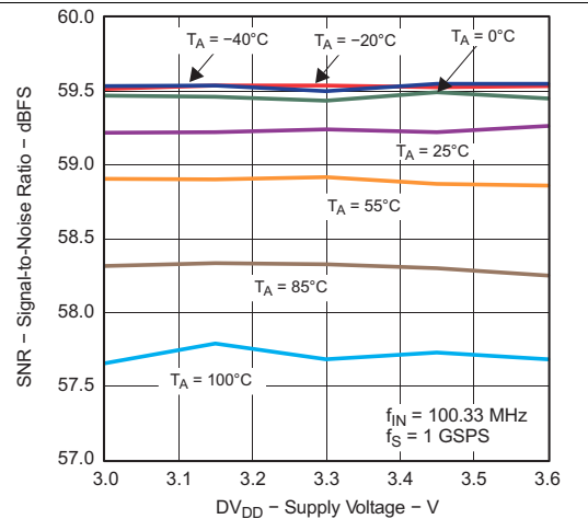
Figure 21. SNR vs DVDD3 Across Temperature
