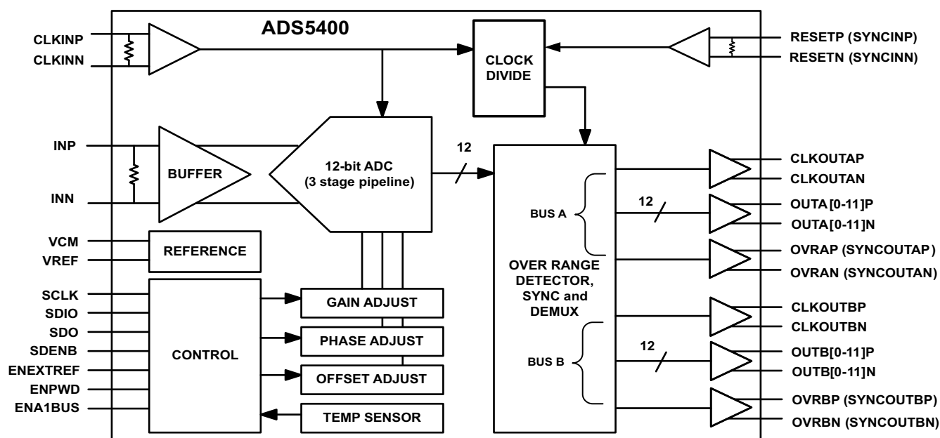
Block Diagram
