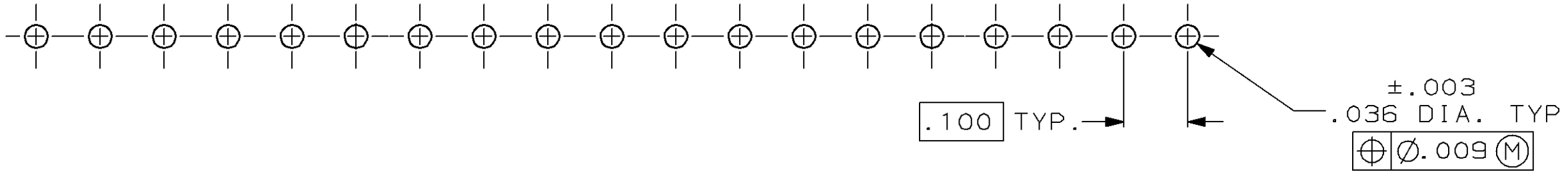
RECOMMENDED MOUNTING HOLE PATTERN
