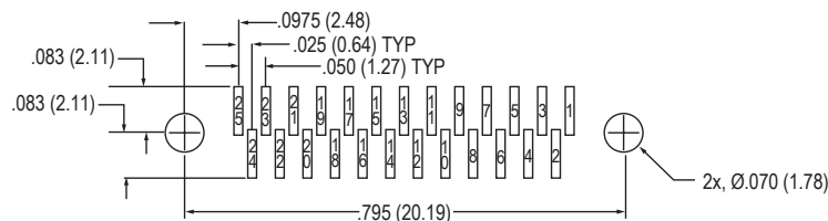
25 Contacts
