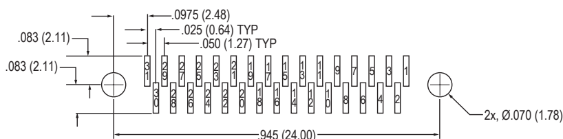
31 Contacts
