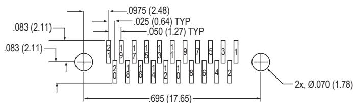
21 Contacts
