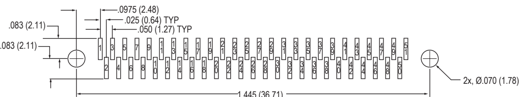
51 Contacts
