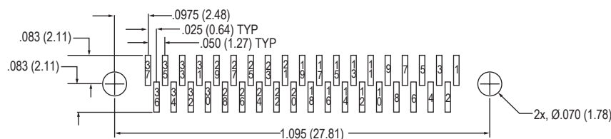
37 Contacts
