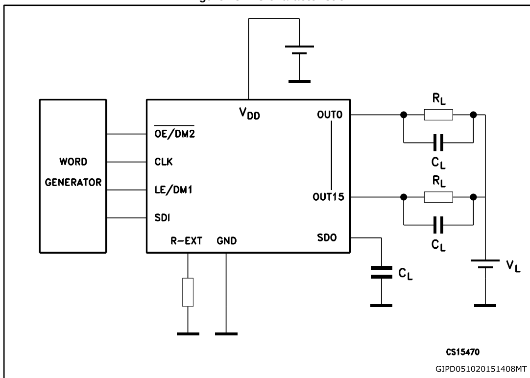
Figure 16: AC characteristic
