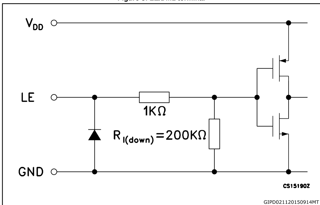
Figure 3: LE/DM1 terminal
