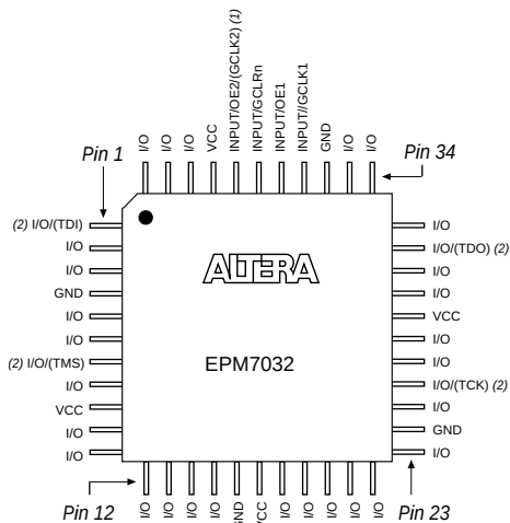
Figure 16. 44-Pin Package Pin-Out Diagram
