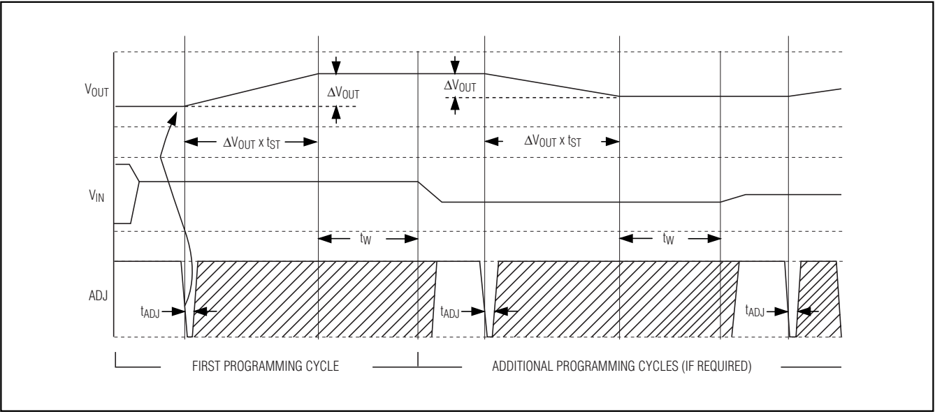
Figure 1. Timing Diagram
