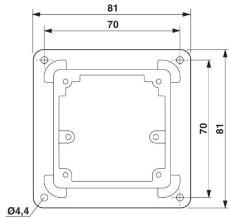
Dimensional drawing
