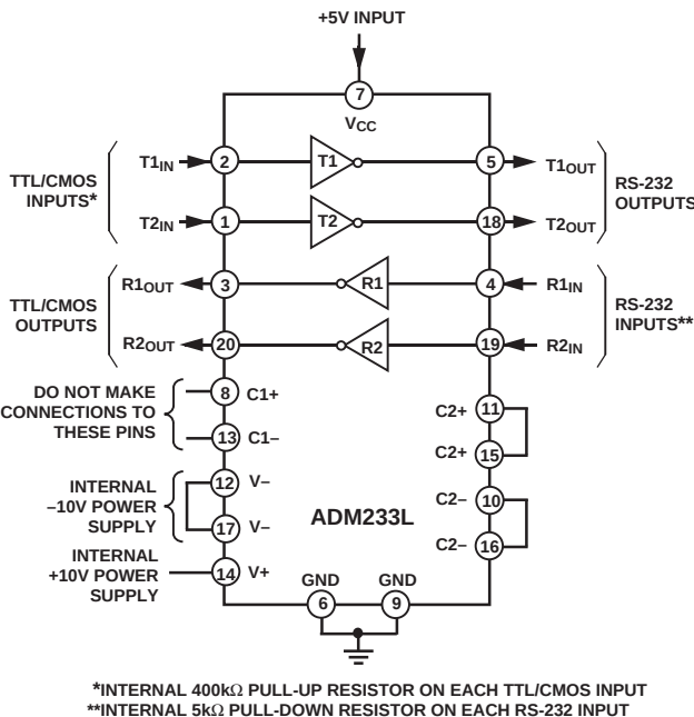
Figure 8. ADM233L Typical Operating Circuit
