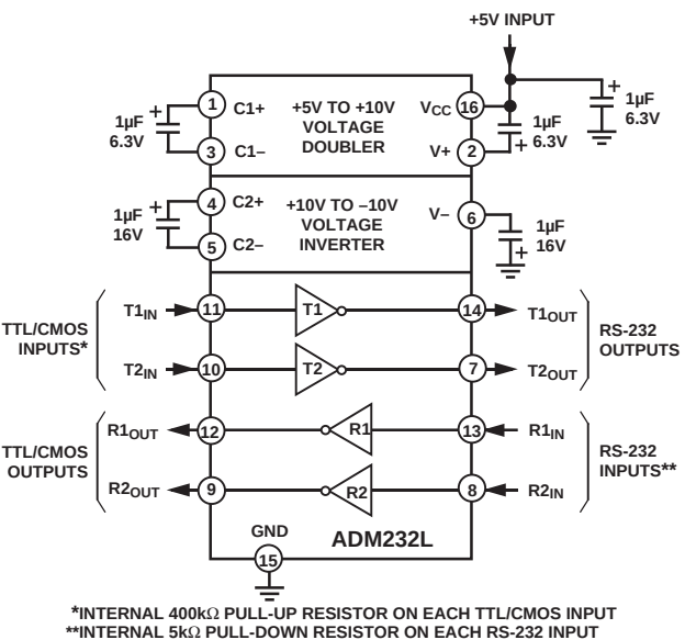
Figure 6. ADM232L Typical Operating Circuit
