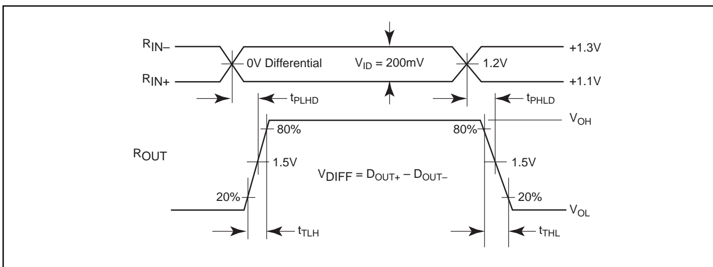
Figure 2. Driver Propagation Delay & Transition Time Waveforms
