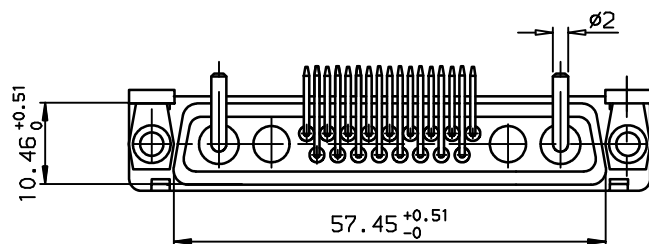
LAYOUT DIMENSIONS (after plating) CONNECTOR SIDE VIEW
