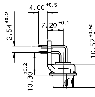
VIEW WITHOUT POWERS CONTACTS
