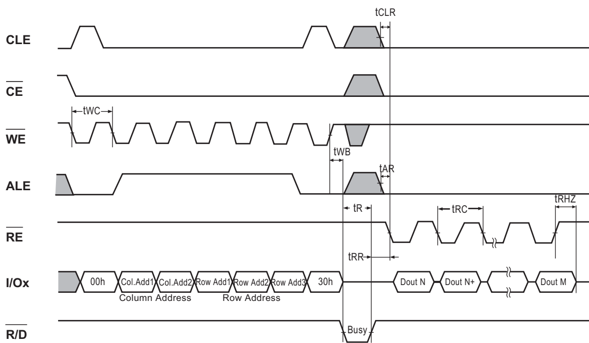
Figure 10: Read1 Operation (Read One Page)
