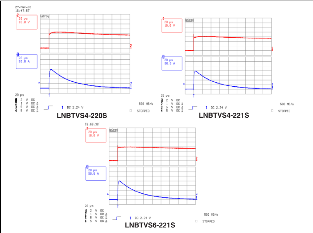
Figure 4. Surge test examples at +4 kV - IEC 61000-4-5, R = 12 \Omega
