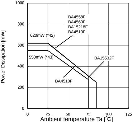
(e)BA4558/BA4560/BA15218/BA15532/BA4510 family
