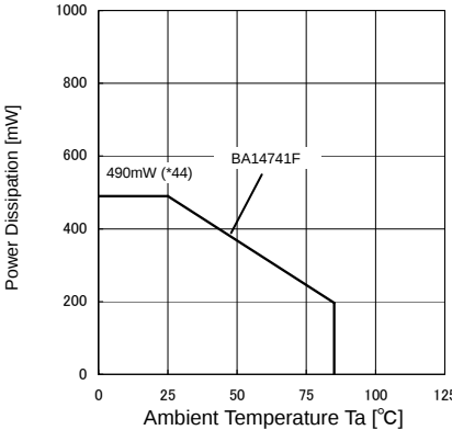
(f)BA14741F
