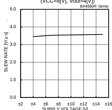
Fig. 84 Slew Rate - Supply Voltage ( C_L=100[pF] , R_L=2[k\Omega] , T_a=25[°C] )
