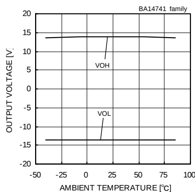
Maximum Output Voltage - Ambient Temperature (VCC/VEE=+15[V]/-15[V], RL=2[kΩ])
