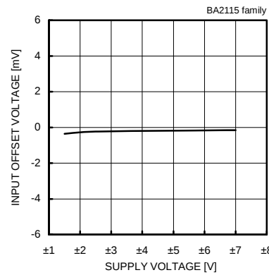
Fig. 296 Input Offset Voltage - Supply Voltage (Vicm=0[V], Vout=0[V])
