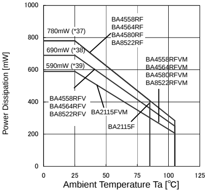
(c)BA4558R/BA4560R/BA4580R/BA8522R/BA2115 family
