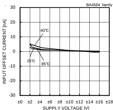
Fig. 145 Input Offset Current - Supply Voltage ( V_{cm}=0[V] , V_{out}=0[V] )
