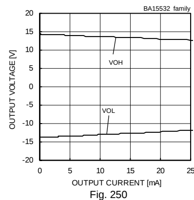
Maximum Output Voltage - Output Current (VCC/VEE=+15[V]/-15[V], Ta=25[°C])
