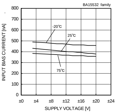
Input Bias Current - Supply Voltage (Vcm=0[V], Vout=0[V])
