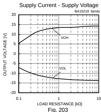
Maximum Output Voltage - Load Resistance (VCC/VEE=+15V/-15V, Ta=25°C)
