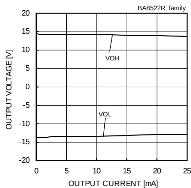
Fig. 184 Maximum Output Voltage - Output Current (VCC/VEE=±15[V]/-15[V], Ta=25[°C])
