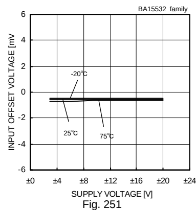
Input Offset Voltage - Supply Voltage (Vcm=0[V], Vout=0[V])
