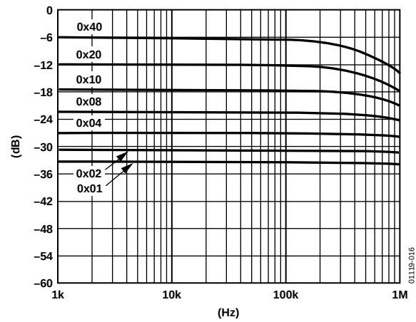
Figure 16. 10 k\Omega Gain vs. Frequency vs. Code
