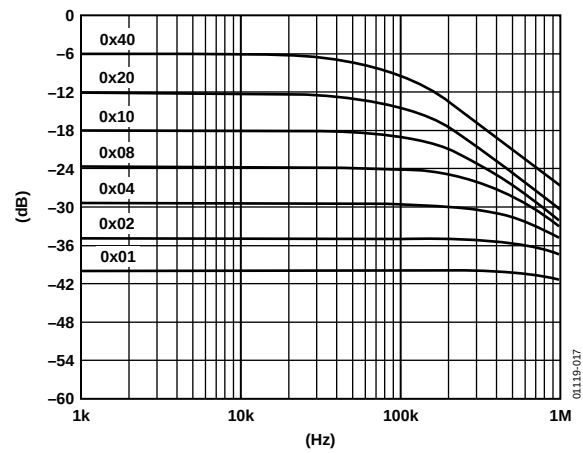
Figure 17. 50 k\Omega Gain vs. Frequency vs. Code
