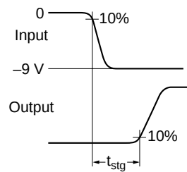
Response Waveform
