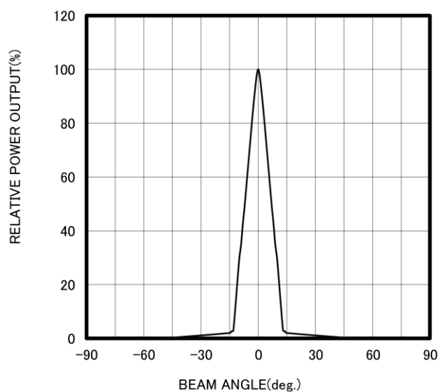
RADIATION PATTERN
