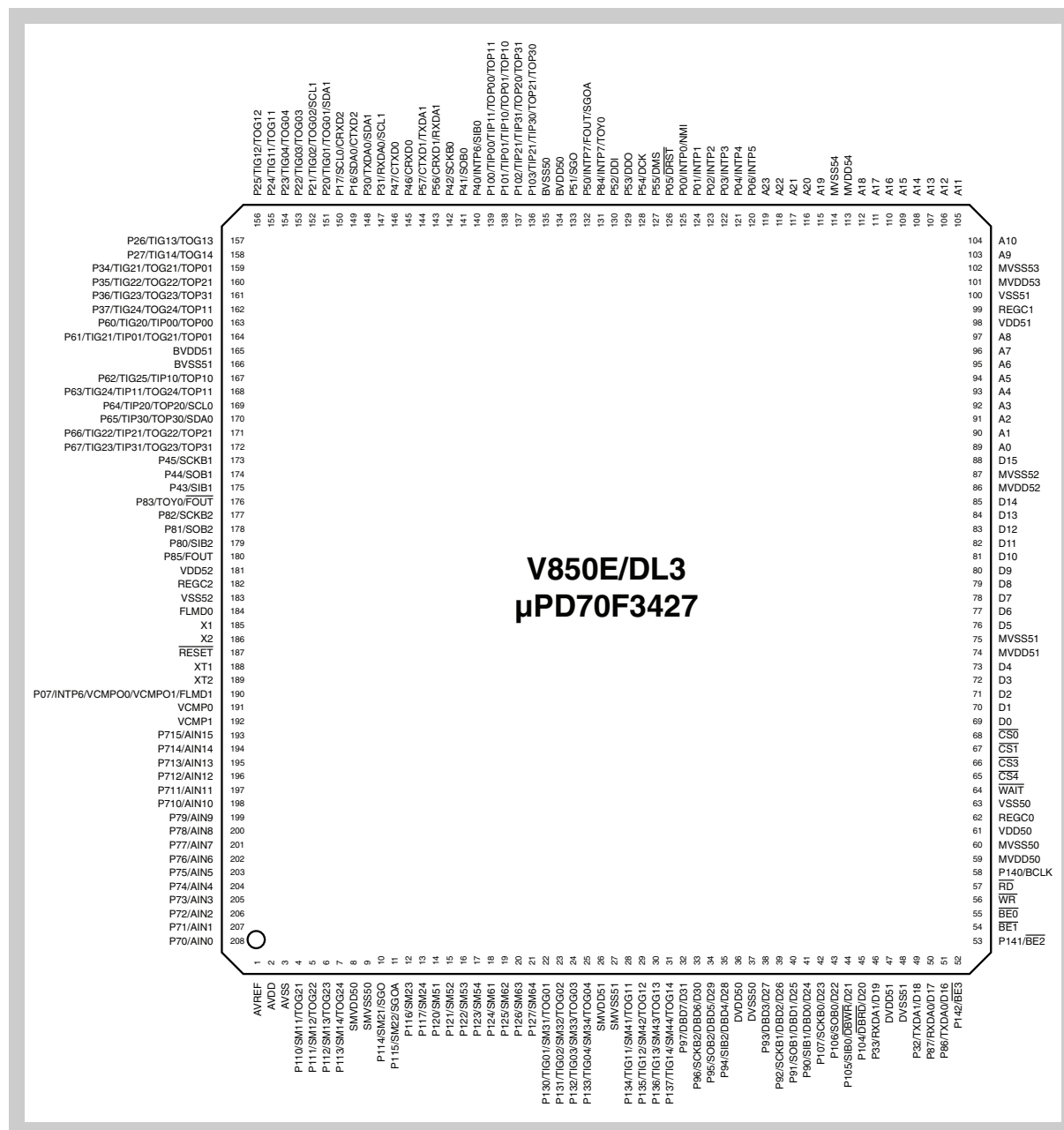
Figure 2-1 Pin Configuration \mu PD70F3427
