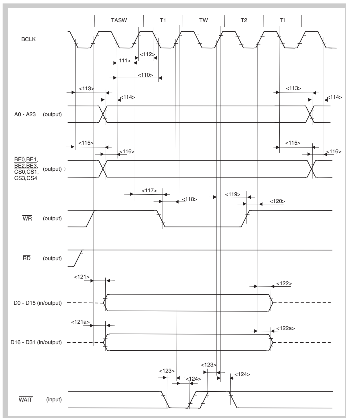
Figure 7-18 External Memory Access Synchronous Write Timing
