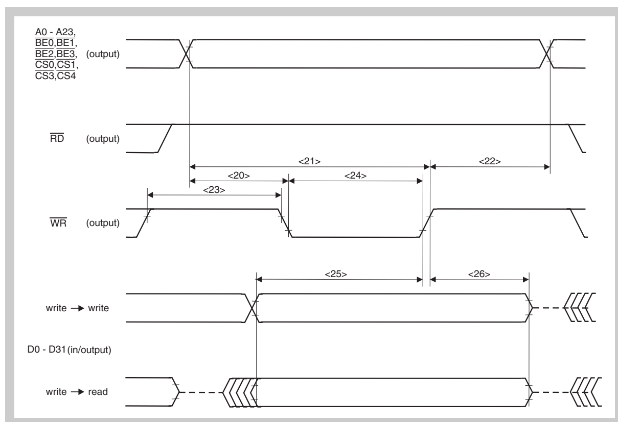
Figure 7-16 SRAM Asynchronous Write Timing
