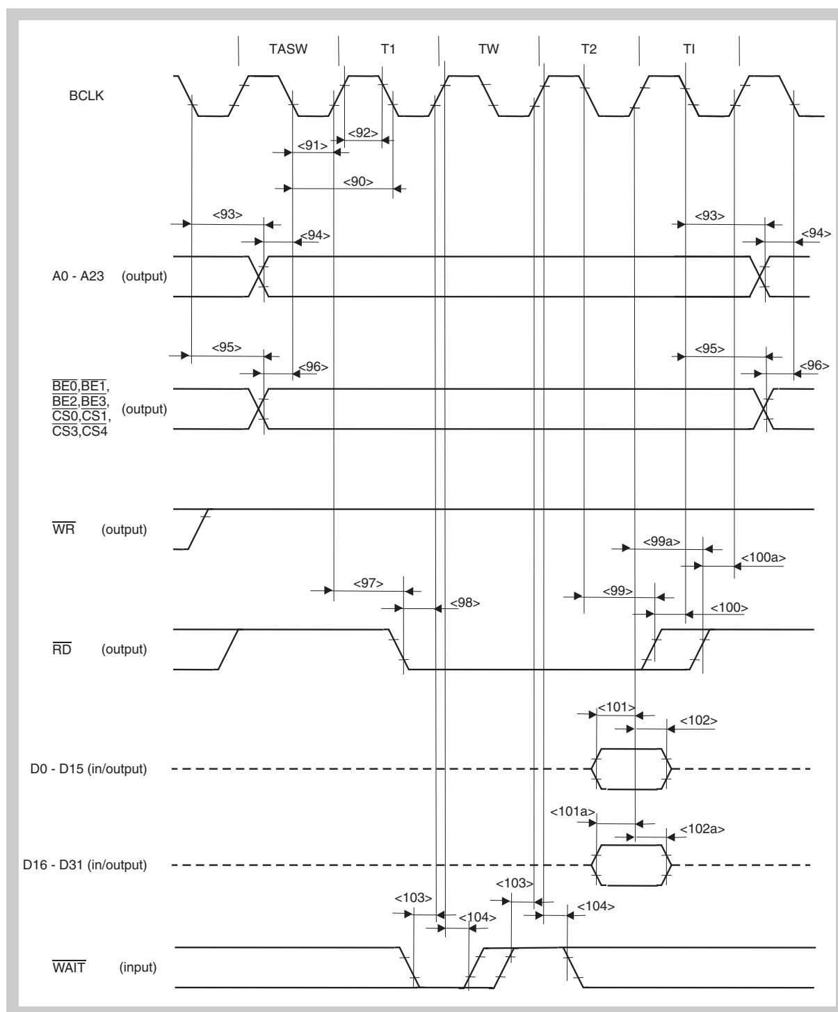
Figure 7-17 External Memory Access Synchronous Read Timing
