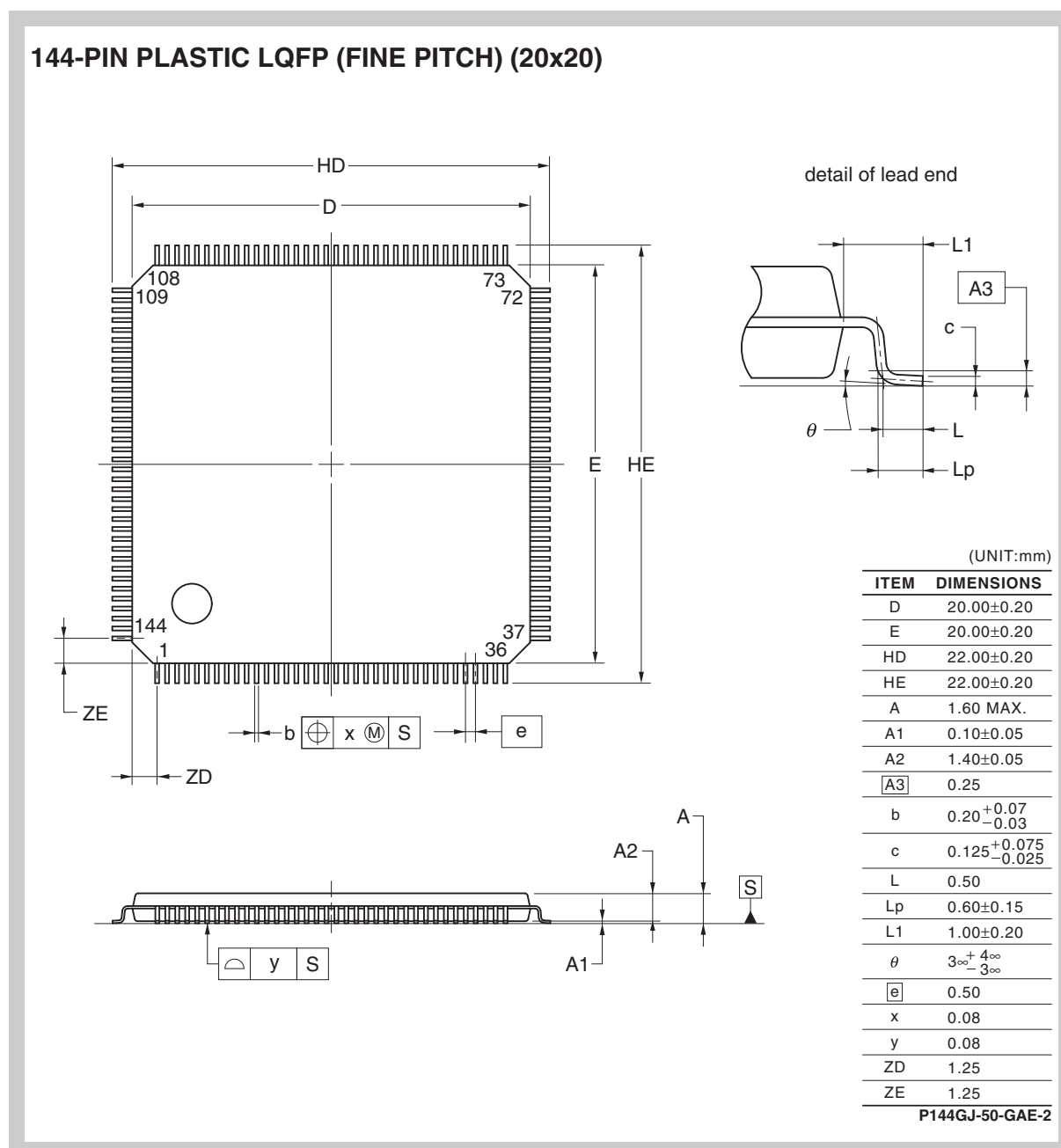
Figure 11-1 Package Drawing of \mu PD70F3426AGJ, \mu PD70F3425GJ, \mu PD70F3424GJ, \mu PD70F3423GJ, \mu PD70F3422GJ, \mu PD70F3421GJ
