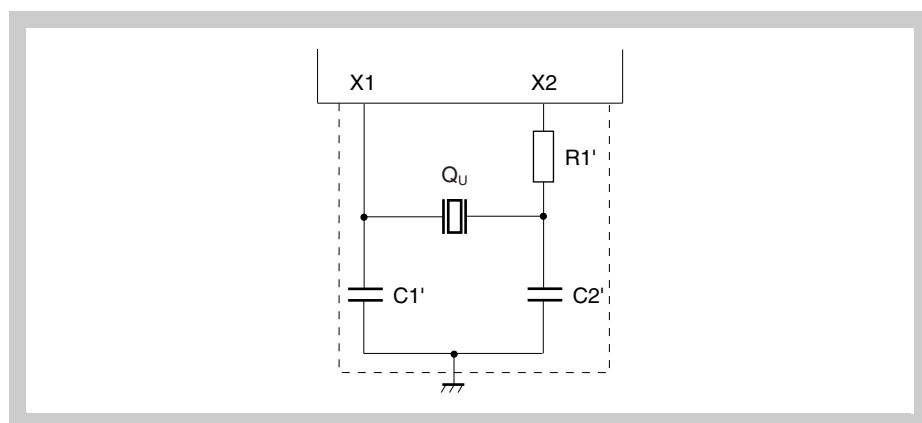
Figure 4-1 Recommended Main Oscillator Circuit
