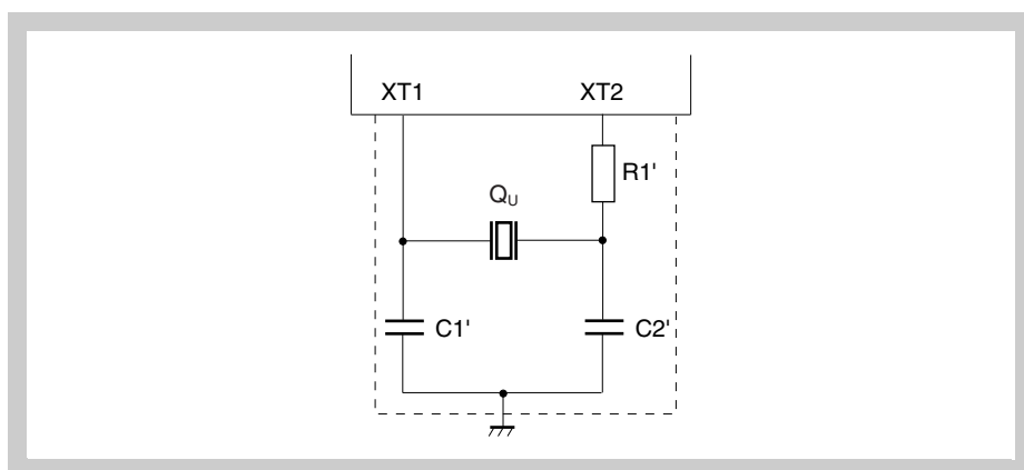
Figure 4-2 Recommended Sub Oscillator Circuit
