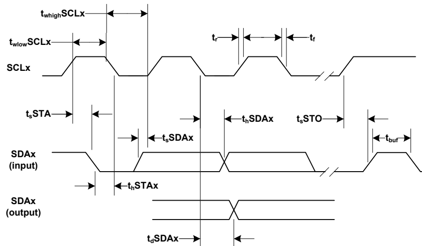
FIGURE 4. 2-WIRE INTERFACE TIMING
