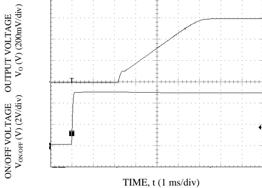
Start-up Using Input Voltage ( V_{IN} = 5V , I_o = I_{o,max} ), V_O = 0.6V
