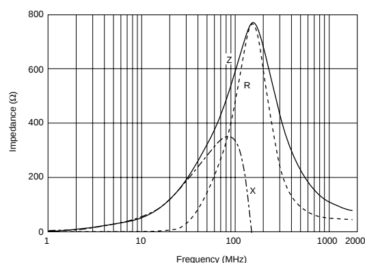
BLM31BE601FN1
