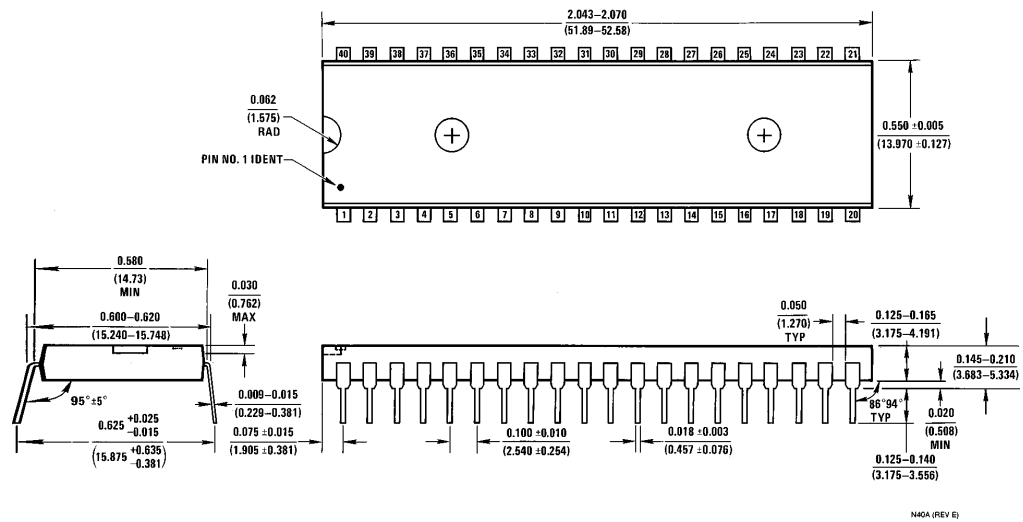
Molded Dual-In-Line Package (N) Order Number COP8780CN NS Package Number N40A
