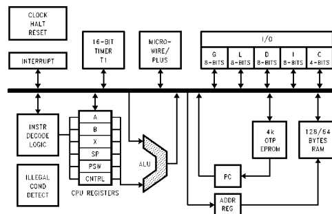
FIGURE 1. Block Diagram
