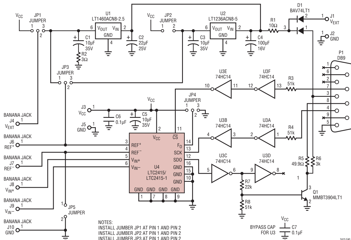
Figure 40. 24-Bit A/D Demo Board Schematic
