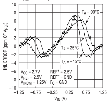
Integral Nonlinearity Over Temperature ( V_{CC} = 2.7V , V_{REF} = 2.5V )
