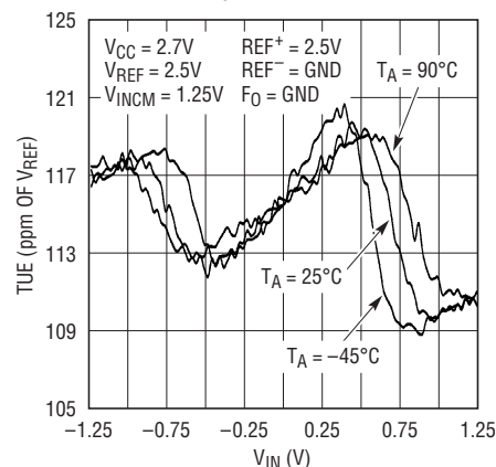
Total Unadjusted Error Over Temperature ( V_{CC} = 2.7V , V_{REF} = 2.5V )
