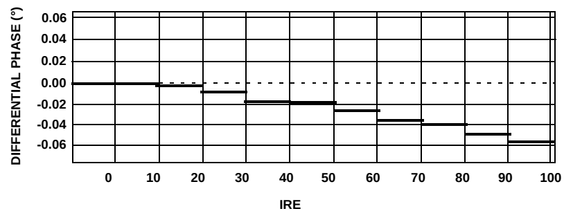
FIGURE 28. DIFFERENTIAL PHASE (°)
