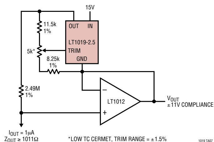
Precision 1 \mu A Current Source
