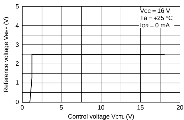
Reference voltage vs. Control voltage
