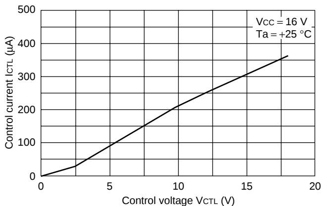
Control current vs. Control voltage
