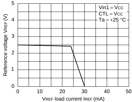
Reference voltage vs. V_{REF} load current
