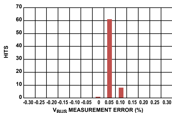
FIGURE 8. V_{BUS} MEASUREMENT ERROR DISTRIBUTION
