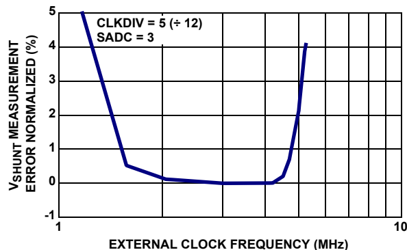
FIGURE 39. EXTERNAL CLOCK BANDWIDTH vs MEASUREMENT ACCURACY
