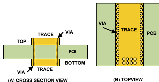
FIGURE 50. ILLUSTRATES A LAYOUT EXAMPLE OF A MULTIPLE LAYER TRACE RESISTOR
