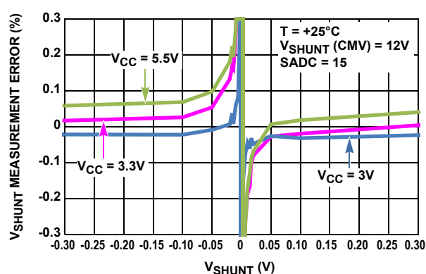
FIGURE 6. V_{SHUNT} MEASUREMENT ERROR vs V_{SHUNT} INPUT
