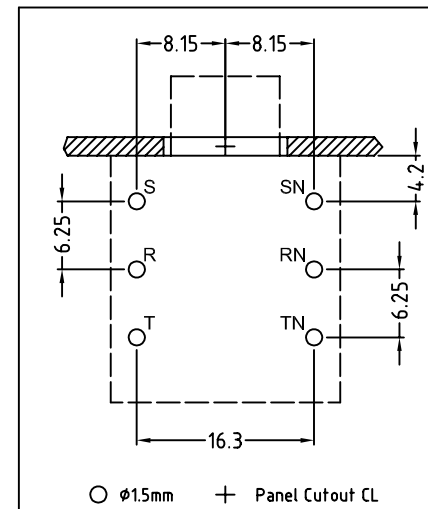
PCB LAYOUT
