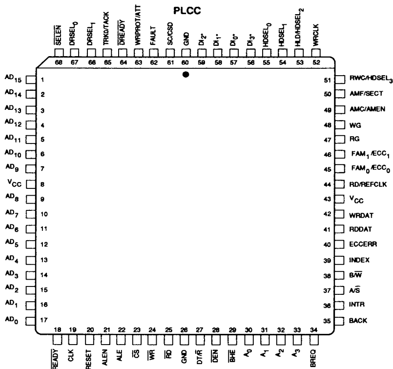
Top View
