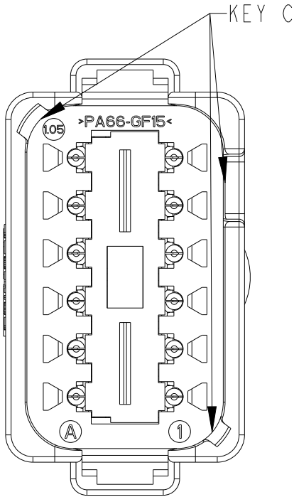
DT04-12PC-P075 HOUSING COLOR: GREEN CAP COLOR: BLACK
