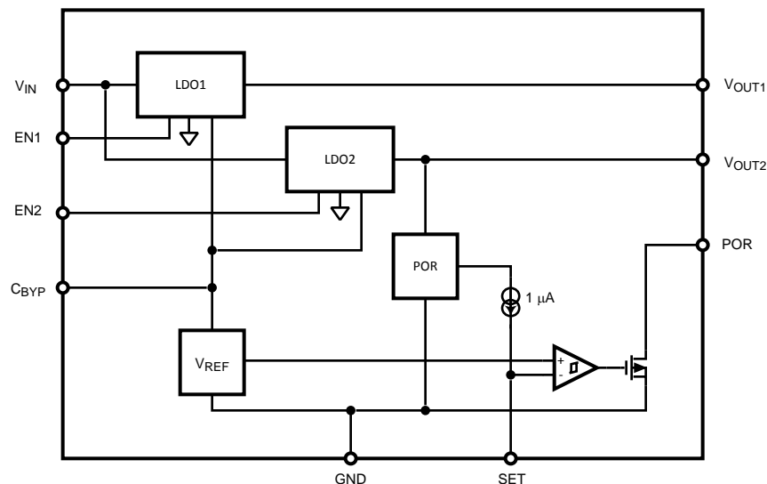
Pin Functions
