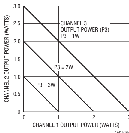
Figure 9. Power Output Capability of an Individual Channel Depends on the Output Power of the Other Channels
