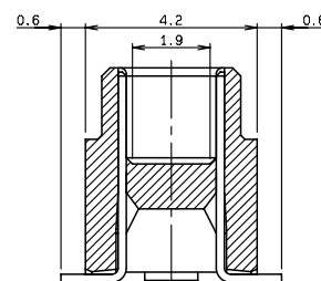
SECT. D-D
