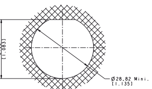
Panel Drilling
