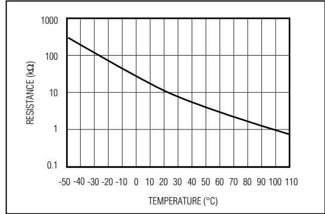
Figure 9. Typical Thermistor Characteristics
