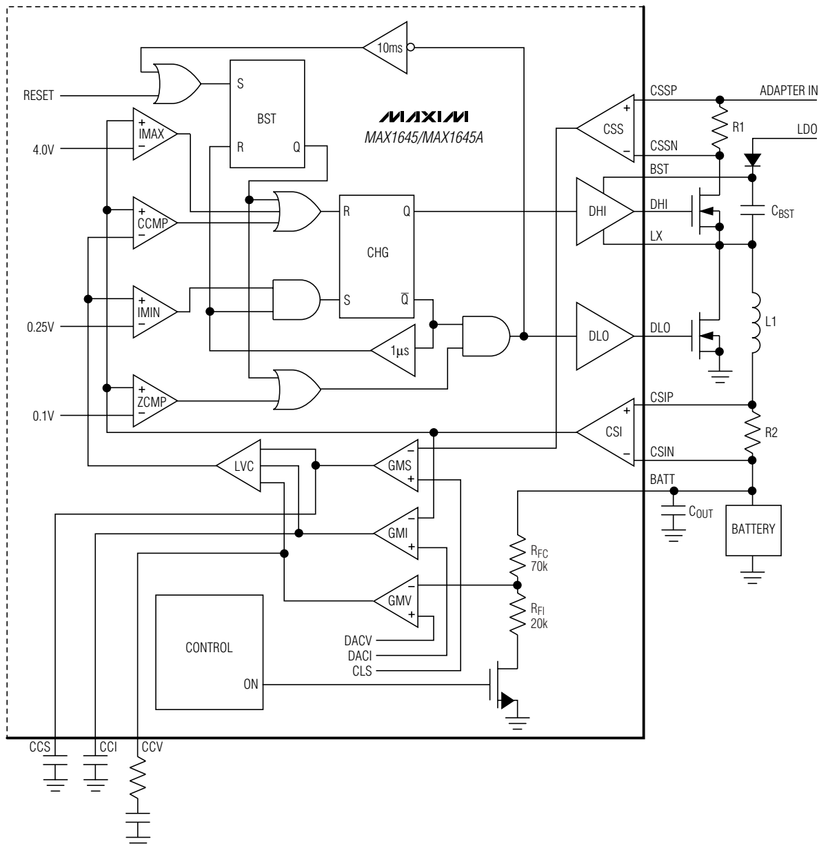
Figure 8. DC-to-DC Converter Functional Diagram
