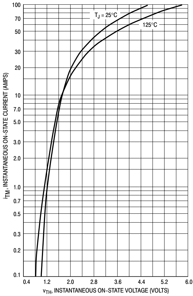
Figure 3. On-State Characteristics
