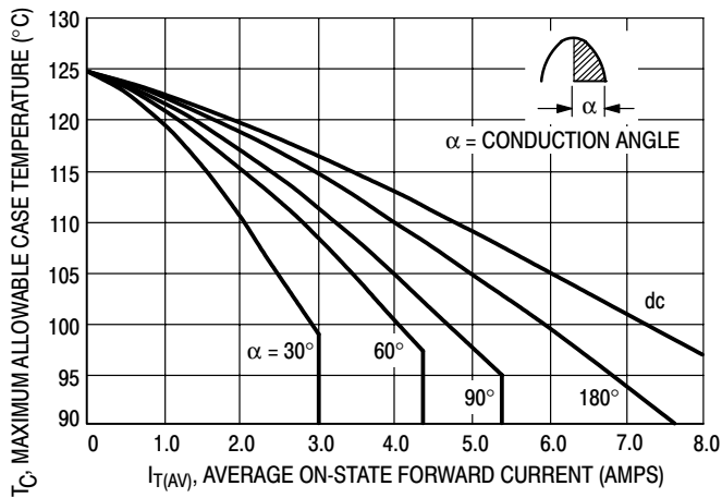
Figure 1. Current Derating
