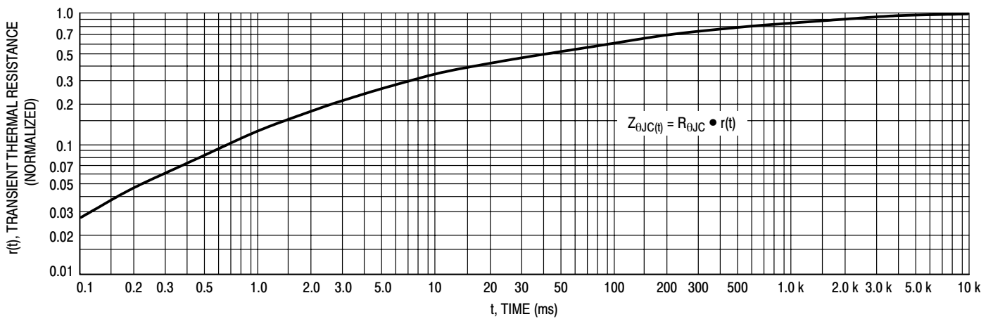
Figure 5. Thermal Response
