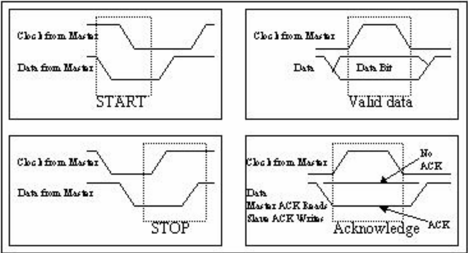
Figure 15: I²C Valid Control Waveforms
