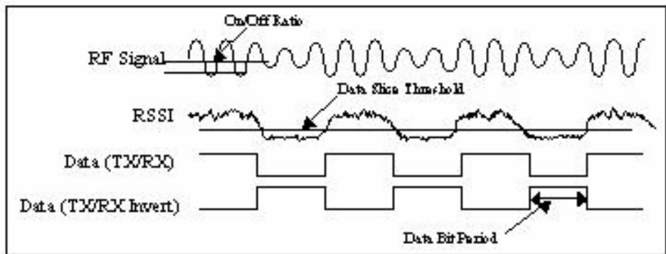
Figure 7: Received Waveform
