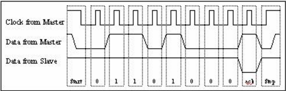
Figure 16: I²C Protocol in a Write 68 (Hex) or a Data Write Request
