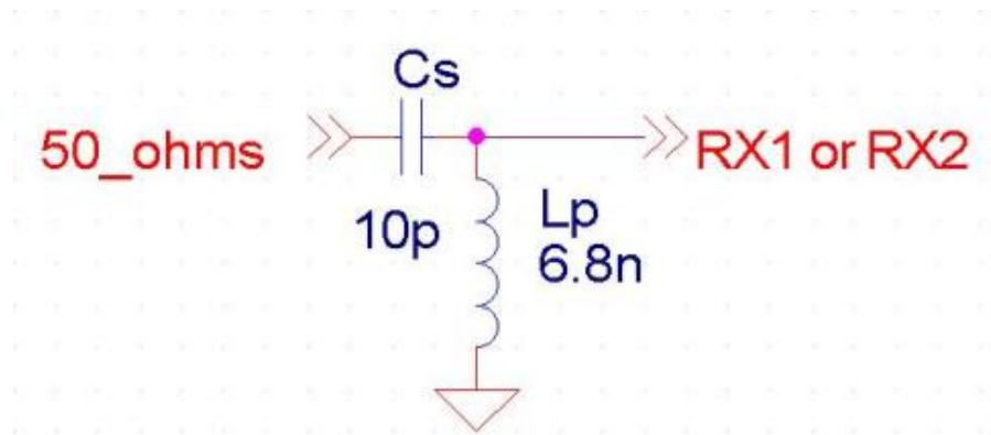
Figure 3: Typical Input Impedance Match to 50Ω (402MHz)
