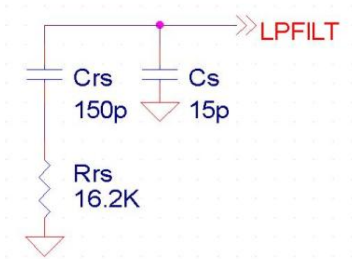
Figure 5: Typical Loop Filter
