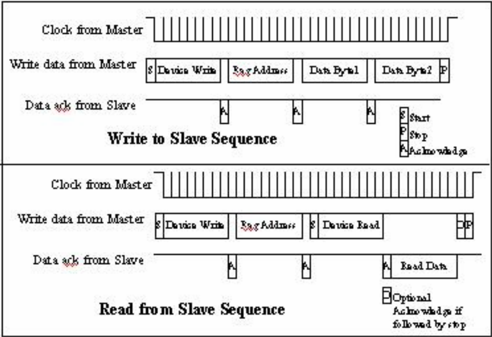
Figure 17: I²C Write and Read Protocol
