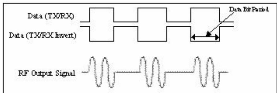
Figure 8: Transmit Waveforms
