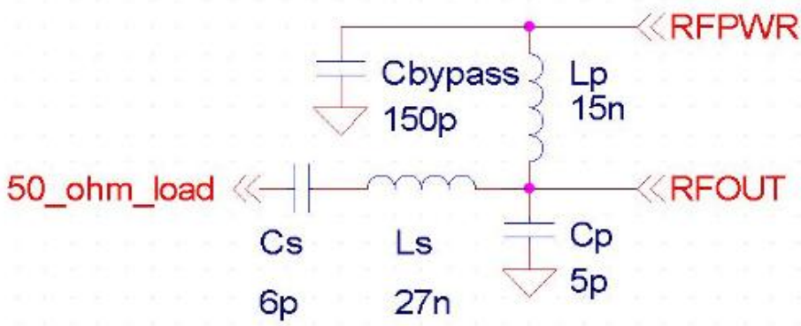
Figure 6: Typical RFOUT Output Impedance Match to 50Ω (402MHz)
