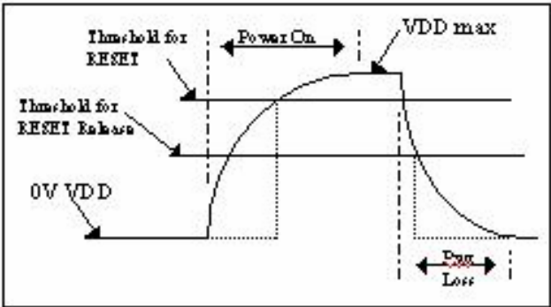
Figure 18: Power-on-Reset Characteristics
