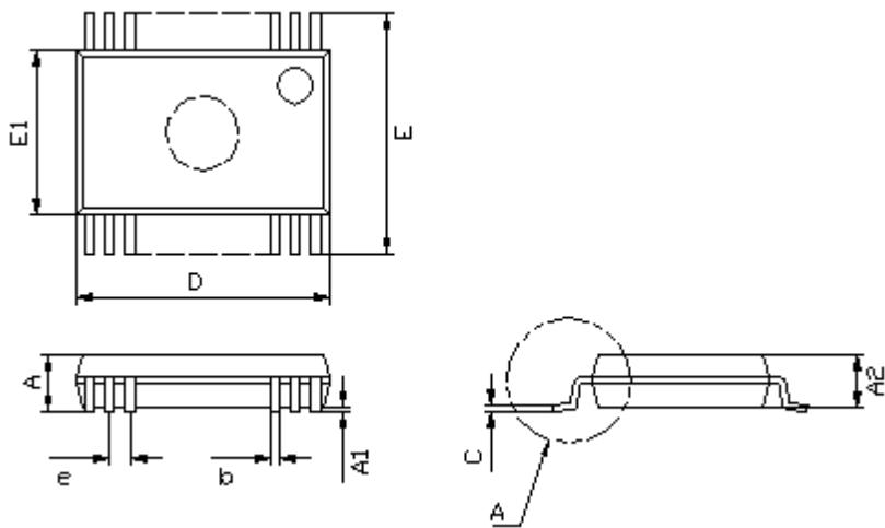
Figure 2: Package Outline
