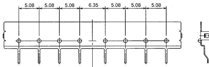
Ground Plate
