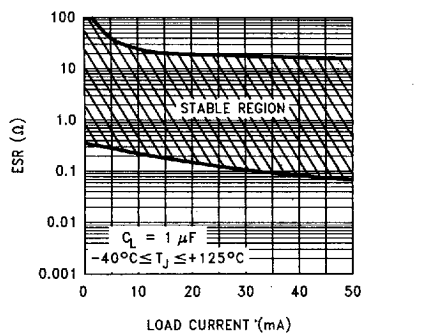
FIGURE 1. 1 \mu F ESR Range
