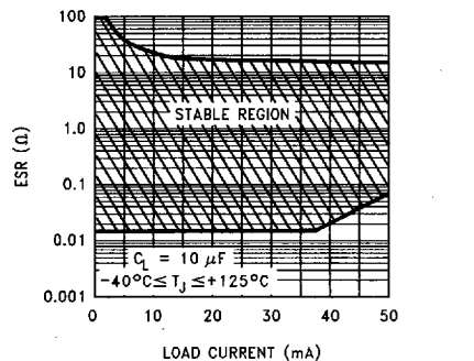
FIGURE 3. 10 \mu F ESR Range
