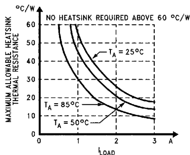
Heatsink Thermal Resistance Requirements
