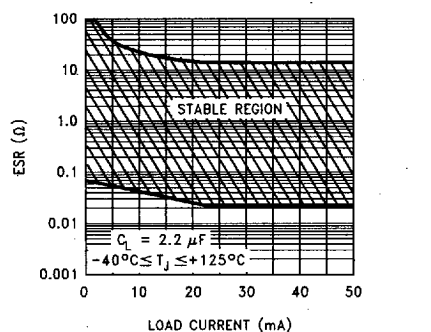
FIGURE 2. 2.2 \mu F ESR Range
