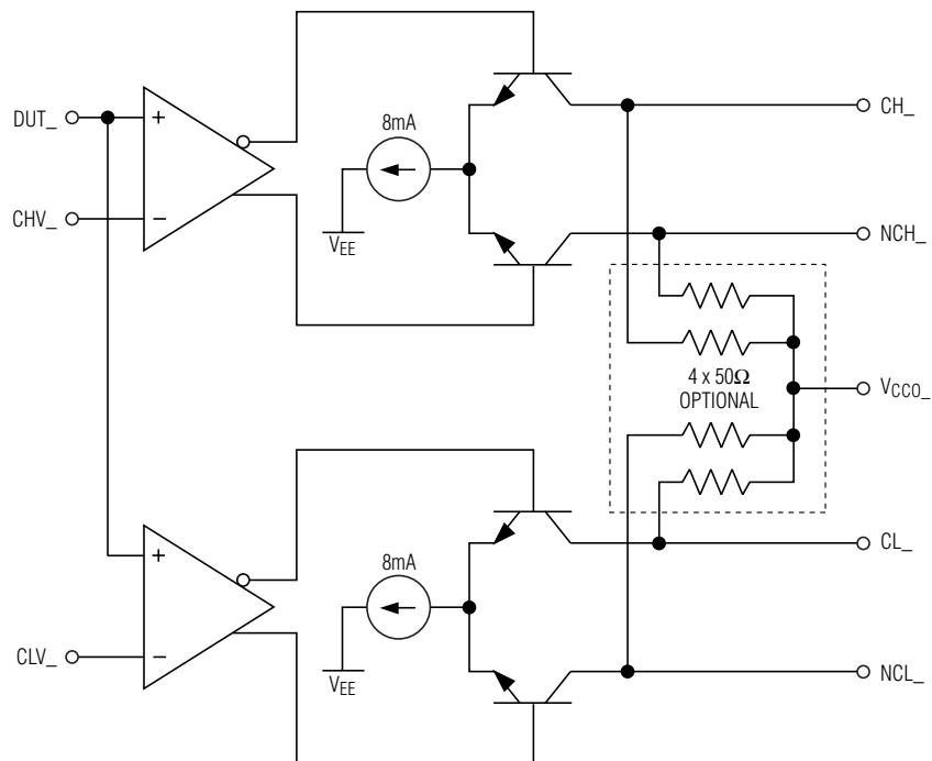
Figure 3. Open-Collector Comparator Outputs
