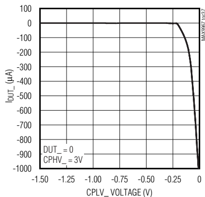
COMPARATOR REFERENCE INPUT CURRENT vs. INPUT VOLTAGE
