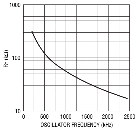
R_T vs Oscillator Frequency
