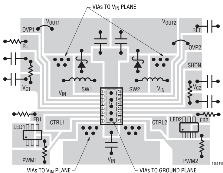
Figure 10. Recommended Layout for LT3486
