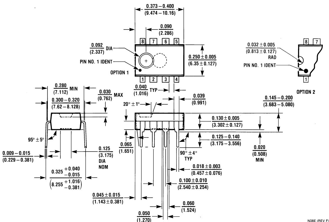
8-Lead (0.300" Wide) Molded Dual-In-Line Package
