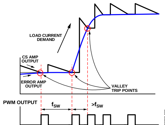
Figure 77. Load Transient Response Operation
