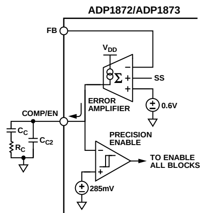
Figure 65. Release COMP/EN Pin to Enable the ADP1872/ADP1873
