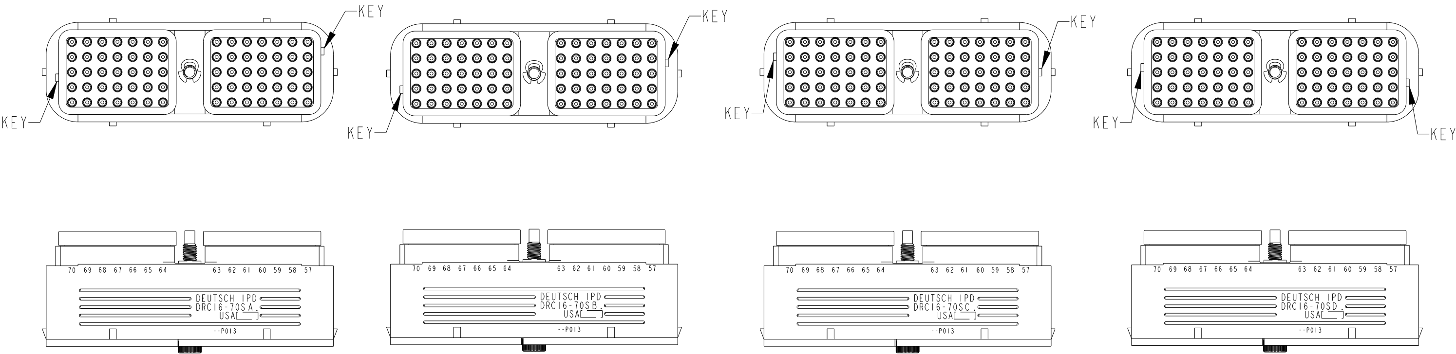
DRC16-70SAE-P013 KEY ARRANGEMENT -A- DRC16-70SBE-P013 KEY ARRANGEMENT -B- DRB16-70SCE-P013 KEY ARRANGEMENT -C- DRC16-70SDE-P013 KEY ARRANGEMENT -D-
