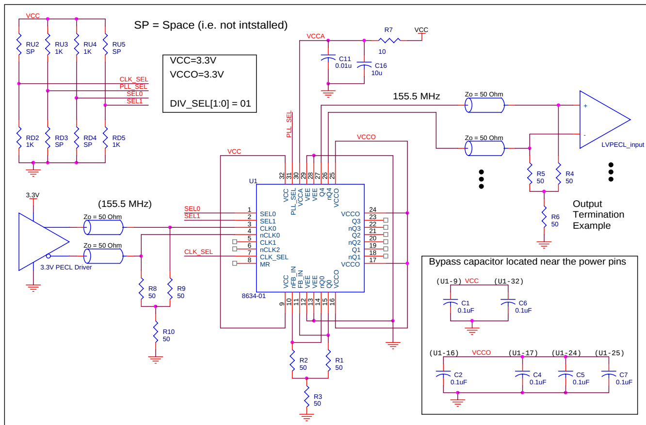
FIGURE 5A. ICS8634-01 LVPECL ZERO DELAY BUFFER SCHEMATIC EXAMPLE
