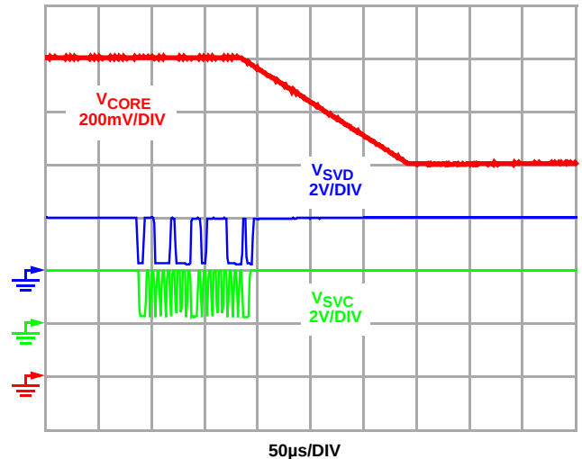
FIGURE 7. CORE SVID TRANSITION: 1.2\text{V} TO 0.8\text{V}
