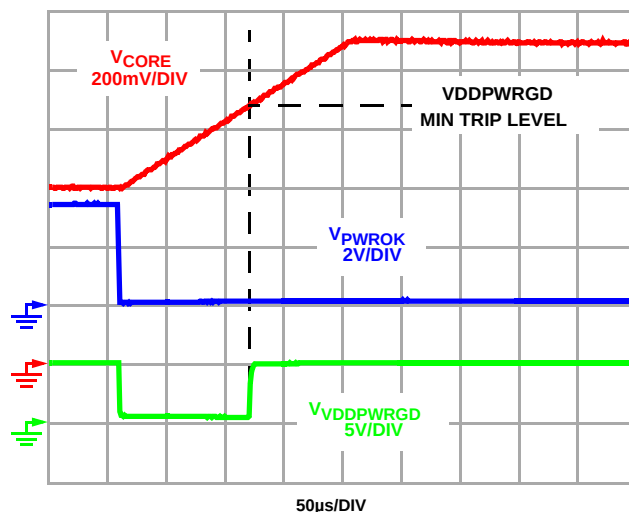
FIGURE 10. CORE VID @ 0.6V; METALVID @ 1.1V
