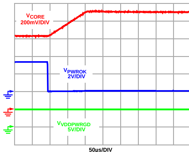
FIGURE 11. CORE VID @ 0.825V; METALVID @ 1.100V
