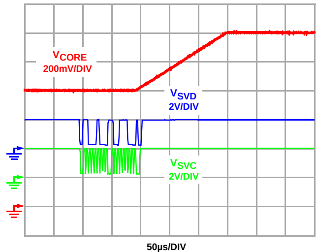
FIGURE 6. CORE SVID TRANSITION: 0.8\text{V} TO 1.2\text{V}
