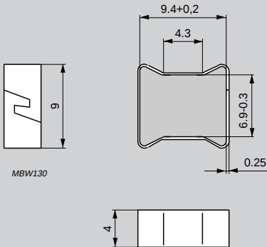
Fig. 2 clip for EP7
