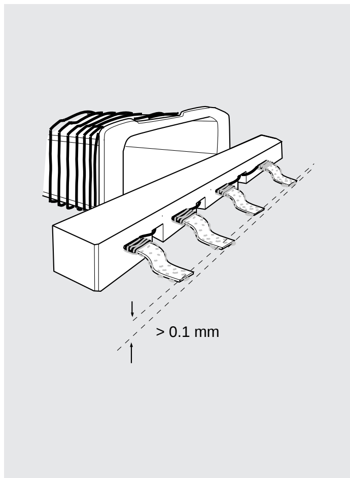
Fig.1 The "gull-wing" design.
