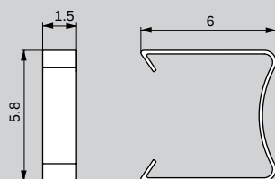
Fig. 2 Clamp for E5.3/2.7/2
