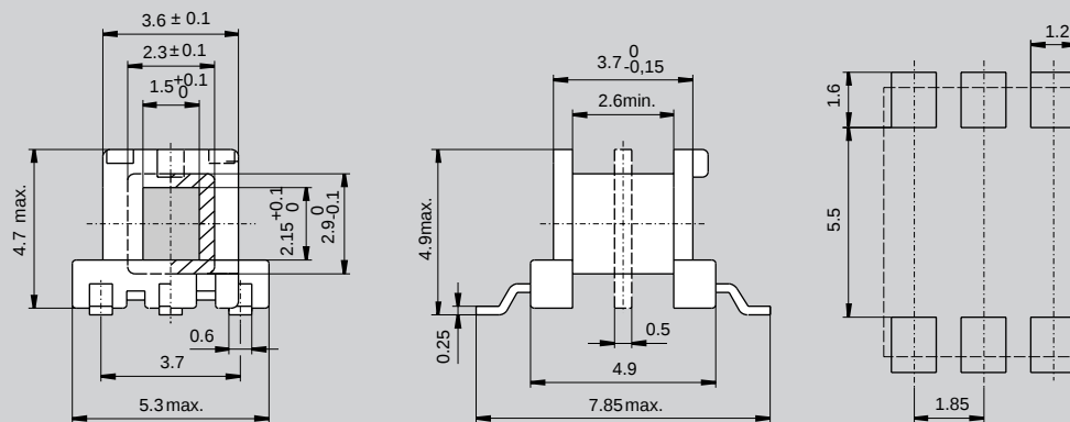
Fig. 1 SMD coil former for E5.3/2.7/2
